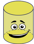
Silindir
